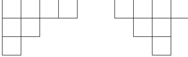
FIGURE 1. \lambda and \mathcal{S}(\lambda) for \lambda = (4, 2, 1)
