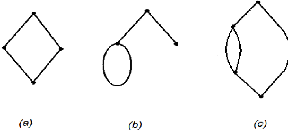
Figure 4: Different examples of the graph \mathbb{G} .
