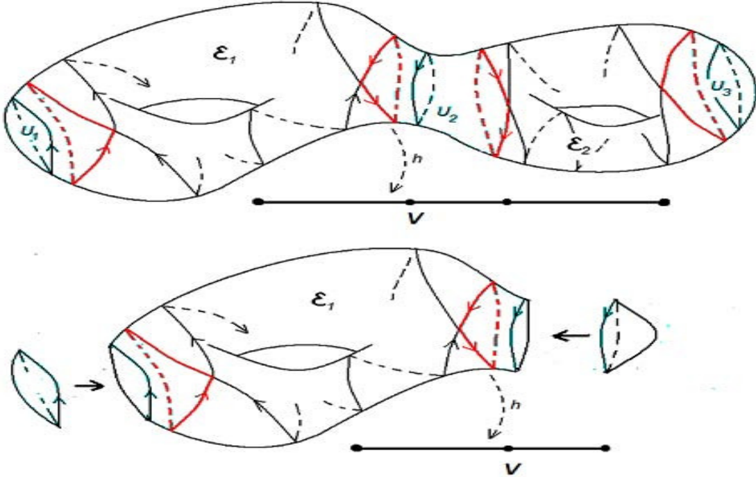
Figure 5: Transition from the surface depicted in Figure 3 to a star-shaped one.
