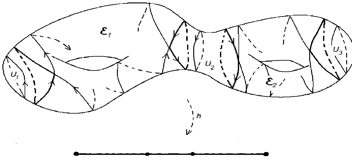
Figure 3: Flow lines on a surface and the corresponding graph \mathbb{G} .
