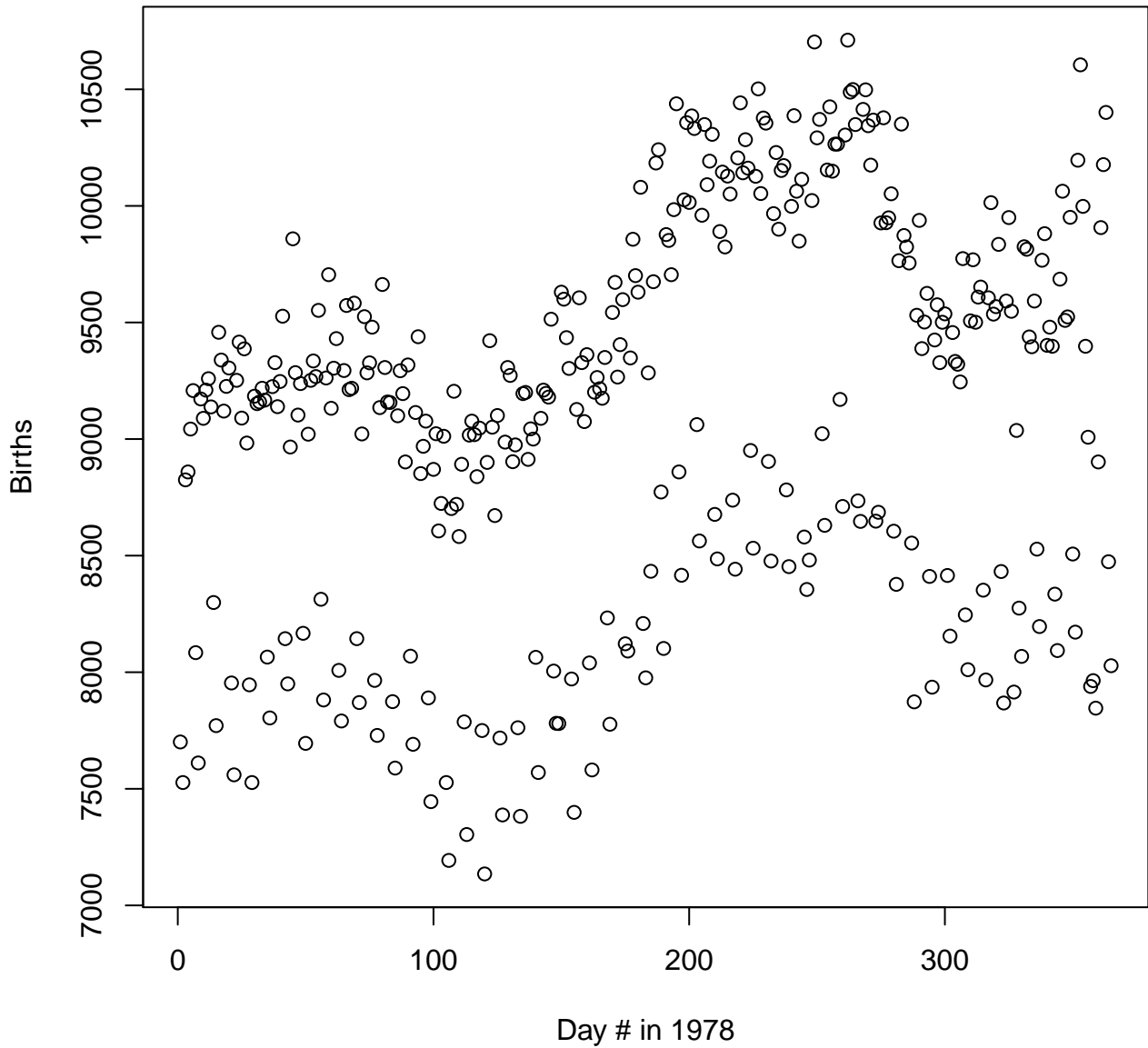
Plot of Births Day by Day in 1978
