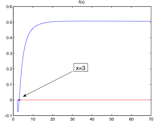
Fig. 2. The function f(x) = \cos^2(\pi/x) - \frac{x-2}{2(x-1)} on [2, 70] .
