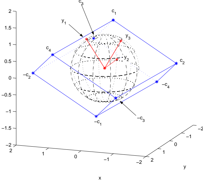
Fig. 3. An example showing the points \pm c_k , k = 1, \dots, 4 , and their relationship to the vectors y_1, y_2, y_3 . Note, y_2 lies on the plane with vertices \{c_1, c_2, -c_3, c_4\} .
