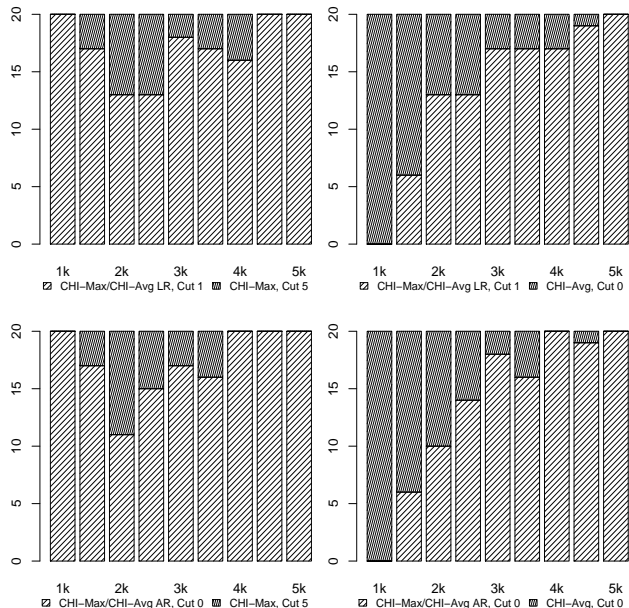
Figure 2: Bars depict how often each method achieved the higher R -precision in 20 trials, comparing combination and non-combination approaches.
