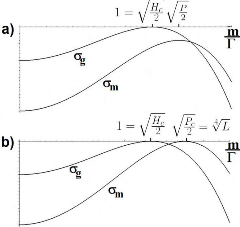
Figure 4: Graphs of \sigma_g = -k^4 + Hk^2 - 1 - \beta (for \beta = 0 ) and \sigma_m = -k^4 + Pk^2 - L , k^2 = l^2 + \frac{m^2}{\Gamma^2} projected on the plane l = 0 , for (a) H = H_c , P < P_c (b) H = H_c , P = P_c , where H_c = 2 and P_c = 2\sqrt[4]{L} are the critical values of H and P .
