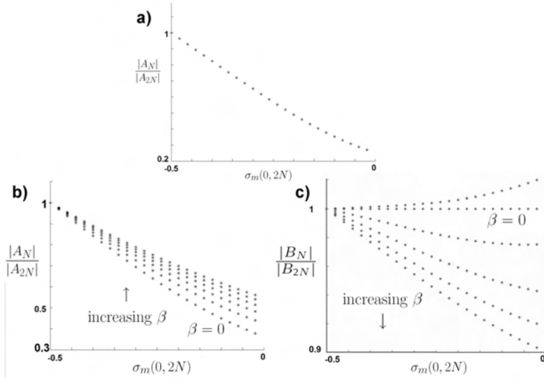
Figure 5: (a) As described in the text, the amplitudes A_N^+ , A_N^- , A_{2N} are found for the case \beta = 0 , C = 0.4 , \kappa = 0.25 , \gamma = 1/15 , L = 1 . Plotted is the ratio |A_N^+|/|A_{2N}| = |A_N^-|/|A_{2N}| as a function of \sigma_m(0, 2N) . (b,c) The effect of the biochemical-mechanical coupling coefficient \beta on the amplitude ratios. For \beta increasing from 0 to positive values, the amplitude ratios |A_N^+|/|A_{2N}| and |B_N^+|/|B_{2N}| are plotted as functions of \sigma_m(0, 2N) . Other parameters are as for part (a).
