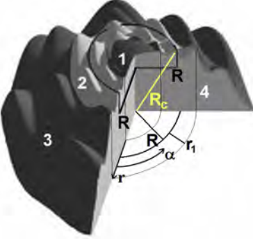
Figure 2: Schematic diagram of the shoot apical meristem (SAM). The SAM consists of a thin skin (the tunica , Regions 1,2,3 in the diagram) attached to a foundation of less well organized cells (the corpus , Region 4). Cells in Region 1 show little growth activity and Region 2 is the generative region in which some active cell division is occurring and new primordia are first seen to form. As the plant tip grows, cells move from Region 2 to Region 3, radially outward in the reference frame of the diagram's north pole. In Region 3, primordia further develop into mature phylla such as leaves. We define radial r and angular \alpha coordinates on the generative region (Region 2) by projecting the surface to polar coordinates on the plane.
