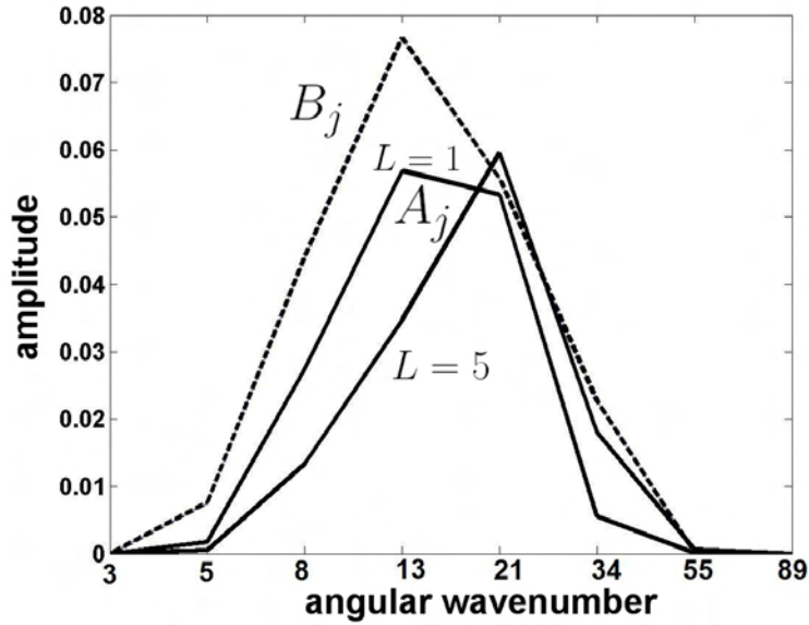
Figure 7: The amplitudes A_j , B_j (vertical axis) vs. angular wavenumber. The amplitude equations for eight modes with angular wavenumbers 3, 5, \dots , 89 are solved as described in the text for the parameter values \Gamma = 19.2 , H = 2.4 , \kappa = 3 , \delta = 0.01 , C = 1 , \gamma = 0.01 , \chi = 0 and i) L = 1 , P = 2.4 , or ii) L = 5 , P = 6 . Plotted are the amplitudes B_j (dotted line) and the amplitudes A_j (solid lines).
