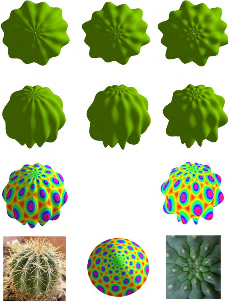
Figure 6: The surface deformation and auxin distribution corresponding to the experiments of Fig. 5a. In the top two rows, the deformation w = A_6^+ \cos(lr + 6\alpha) + A_6^- \cos(-lr + 6\alpha) + A_{12} \cos(12\alpha) is plotted as a deformation of the sphere for A_6^\pm/A_{12} = 1/3 (first column, corresponding to \sigma_m = 0 in Fig. 5a), A_6^\pm/A_{12} = 2/3 (second column, corresponding to \sigma_m = -1/3 in Fig. 5a) and A_6^\pm/A_{12} = 1 (third column, corresponding to \sigma_m = -1/2 in Fig. 5a). The auxin distribution is plotted in the third row together with the surface deformation and in the center of the fourth row by itself; plotted is g = B_6^+ \cos(lr + 6\alpha) + B_6^- \cos(-lr + 6\alpha) + B_{12} \cos(12\alpha) with B_6^+ = B_6^- = B_{12} . Pictured also in the fourth row are plants that show similar surface deformations.
