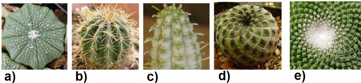
Figure 1: Examples of various phyllotactic lattice and tiling patterns. Ridges (a), undulating ridges (b), hexagons (c), diamonds (parallelograms) (d) and offset diamonds (e) are observed on these succulents. In (d) and (e), the phylla are arranged on families of spirals—families of 8 clockwise and 13 counterclockwise spirals in (d) and 13 clockwise and 21 counterclockwise spirals in (e).
